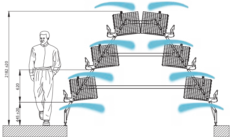
SuperTripleDeck for tropical climates: the air can flow through the system without obstructions
